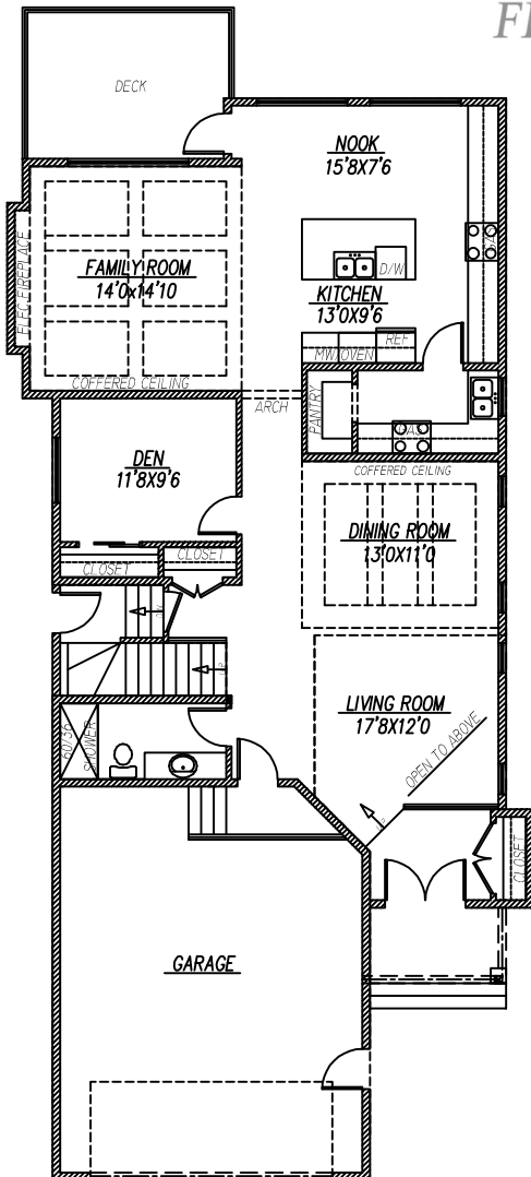
MAIN FLOOR PLAN 1459 SQ. FT.
