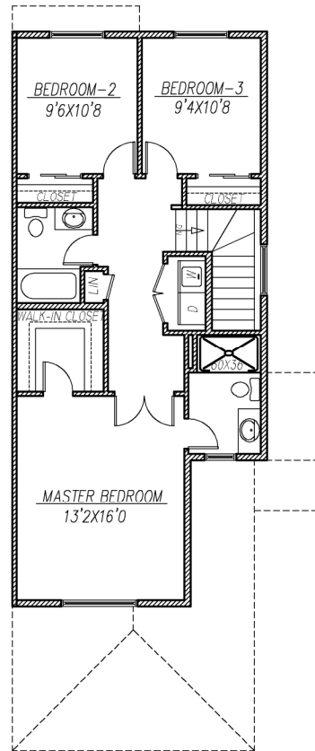
UPPER FLOOR PLAN 784 SQ. FT
