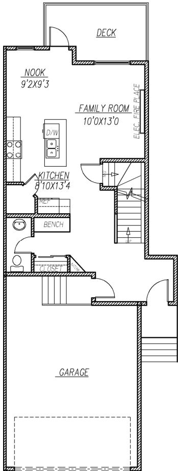
MAIN FLOOR PLAN 672 SQ. FT.
