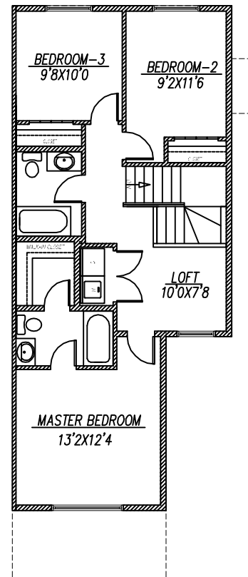
UPPER FLOOR PLAN 768 SQ. FT
